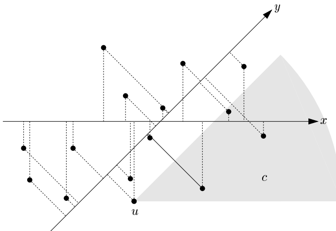
Figure 2: Finding the neighbour of u in c is equivalent to finding the point in the upper right quadrant of u with minimum y coordinate.
