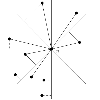
Figure 1: The \theta -cones of v .
