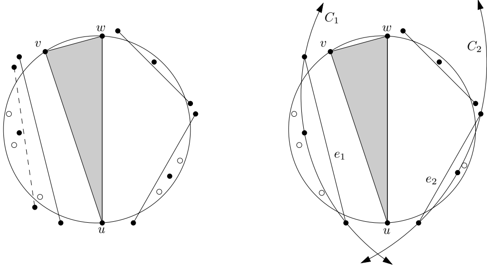
Fig. 2. The order of a triangle in a constrained Delaunay triangulation.
