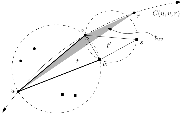
Fig. 3. Illustration of the fact that if \triangle uvs and \triangle uws are not in the triangulation, it must have order at least four.
