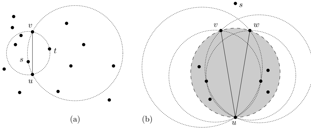
Fig. 1. (a) Illustration of the first-points-hit ( s and t ). (b) Illustration of the proof.
